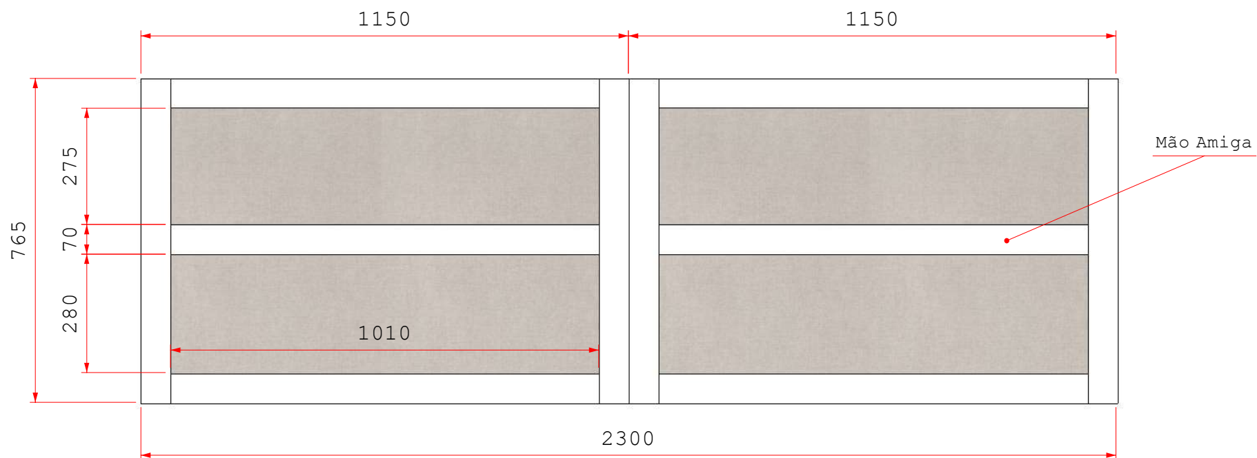
Vista B - Painel TV
