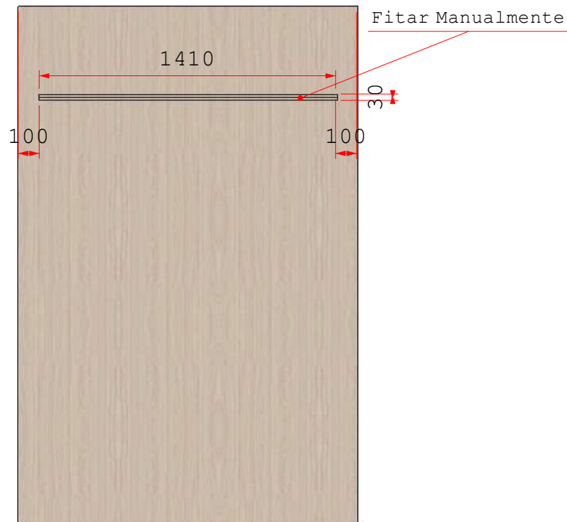
Vista B - Painel TV
