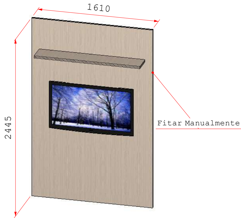
Vista B - Painel TV
