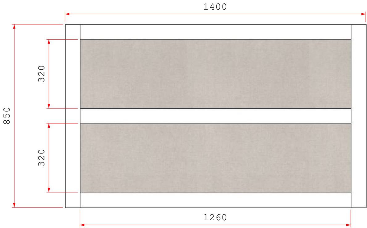
Vista B - Painel TV
