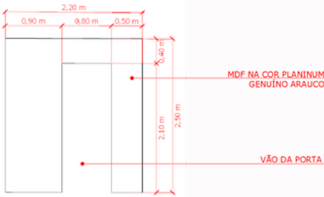
VISTA FRONTAL
