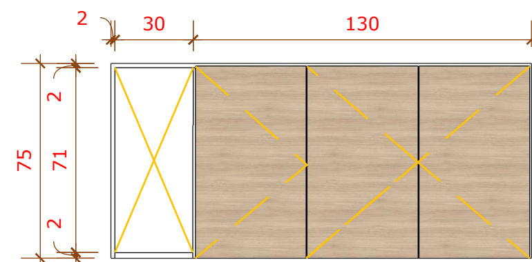
05 VISTA FRONTAL ARM. BALCÃO 1/20
