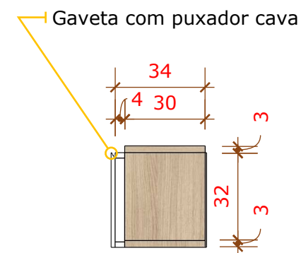
02 VISTA LATERAL RACK 1/20
