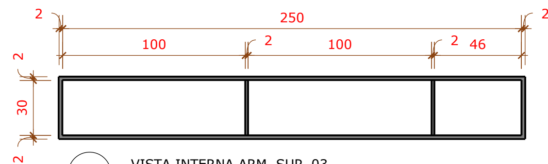
03 VISTA INTERNA ARM. SUP. 03 1/20
