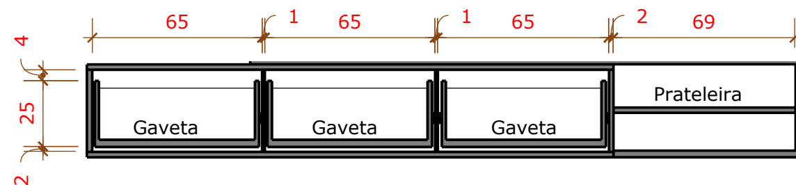
04 VISTA INTERNA RACK 1/20
