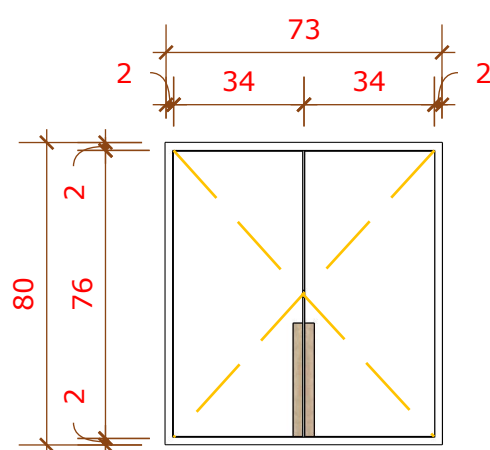
04 VISTA FRONTAL ARM. SUP. 1/20
