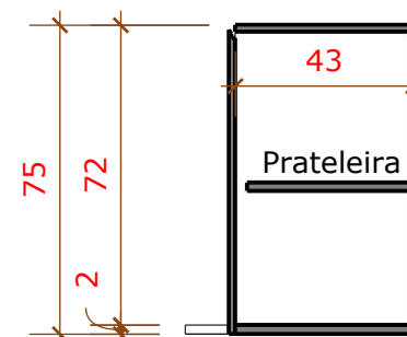
08 VISTA LATERAL ARM. BALCÃO 1/20
