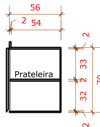
02 CORTE LATERAL ARM. SUP. 01 1/25
