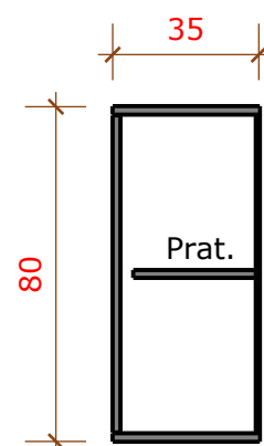
05 CORTE LATERAL ARM. SUP. 1/20
