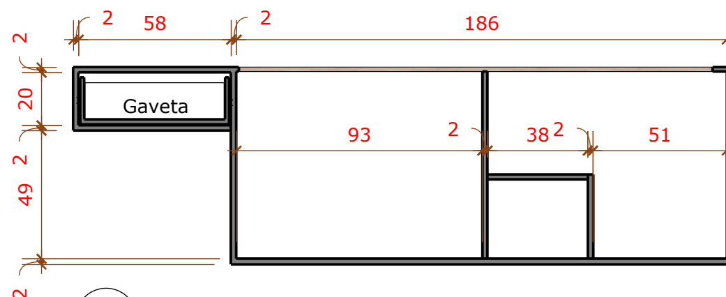
07 VISTA INTERNA ARM. BANCADA 1/20
