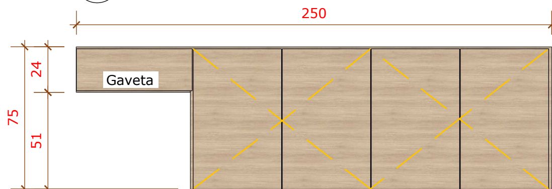
05 VISTA SUPERIOR ARM. BANCADA 1/20
