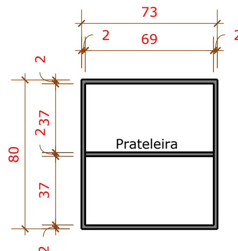
06 VISTA INTERNA ARM. SUP. 1/20
