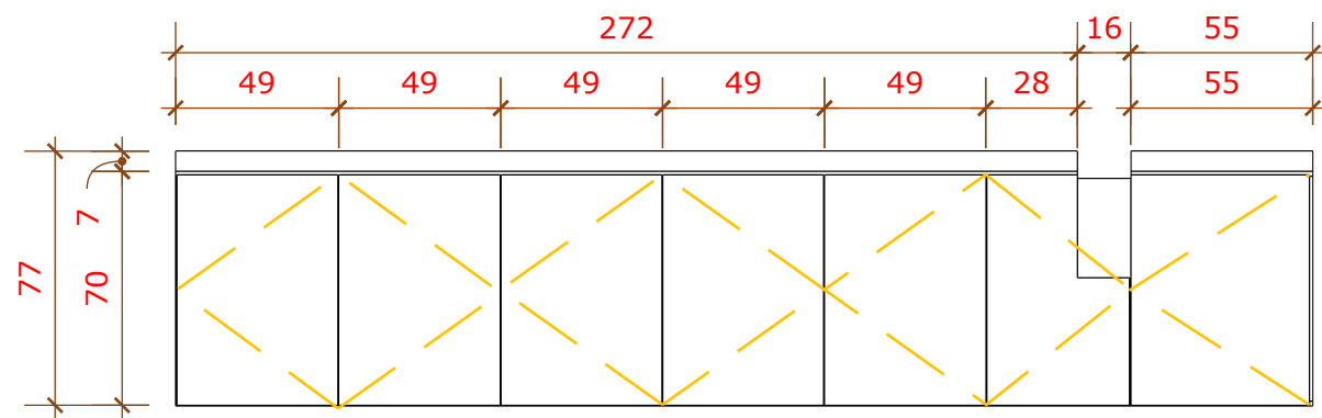
01 VISTA FRONTAL ARM. SUP. 01 1/25
