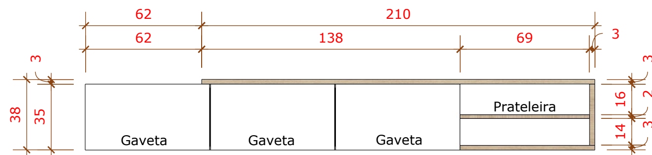
01 VISTA FRONTAL RACK 1/20
