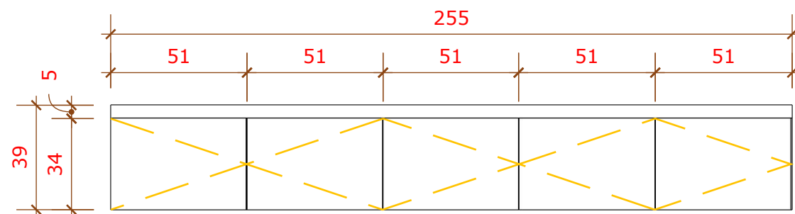
01 VISTA FRONTAL ARM. SUP. 03 1/20
