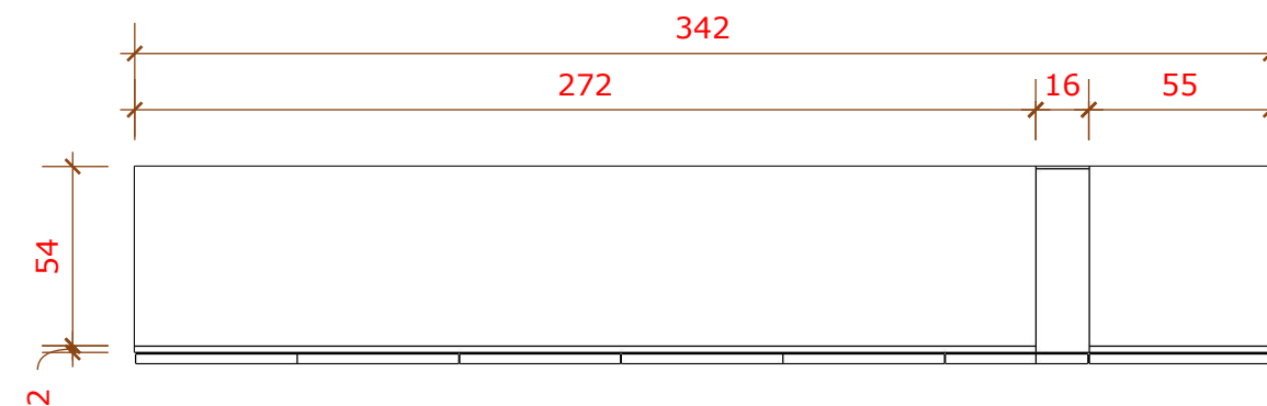
03 VISTA SUPERIOR ARM. SUP. 01 1/25
