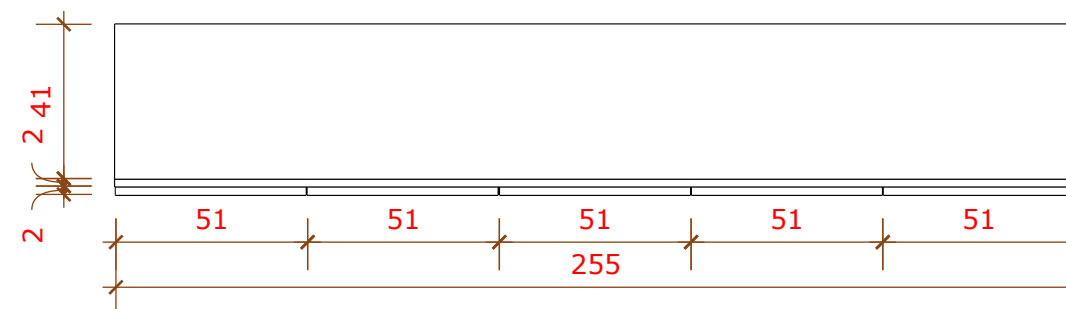
04 VISTA SUPERIOR ARM. SUP. 03 1/20
