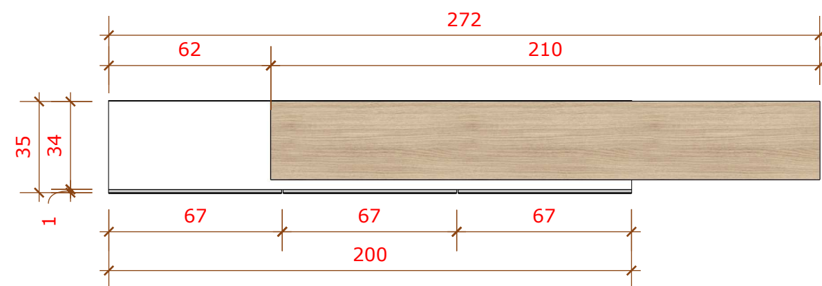
03 VISTA SUPERIOR RACK 1/20
