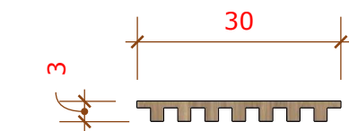
01 VISTA FRONTAL PAINEL 1/10
