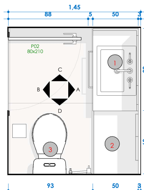
LAYOUT ESCALA 1:25
