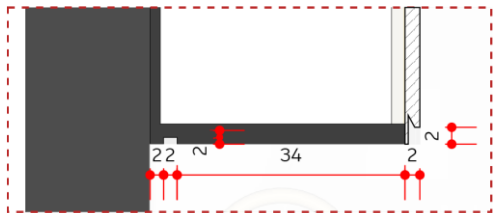
DET 14 | LED Esc 1/10
