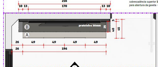
PLANTA | rack + painel TV Esc 1/20
